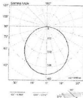
LED PANEL 24W
